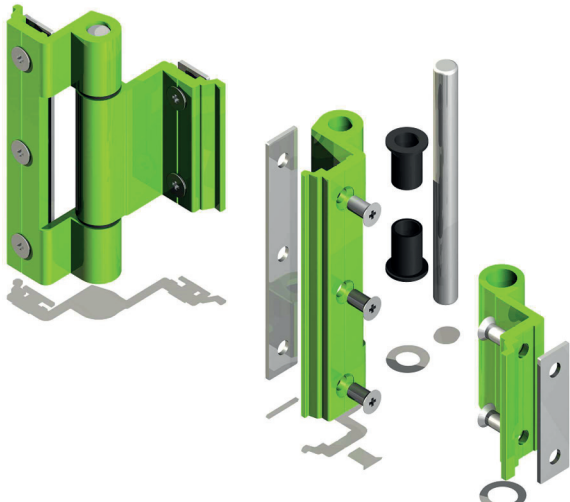
KRC-3305 Alutech pencere-kapı menteşe Window-door hinge Euro Section-kanal 1
