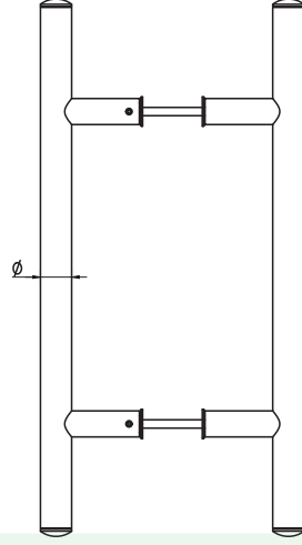
"H" kol "H" pull handle
