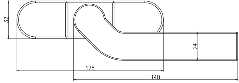
KRC-1704 Tek maçalı cephe kolu Hidden sash window handle single plate
