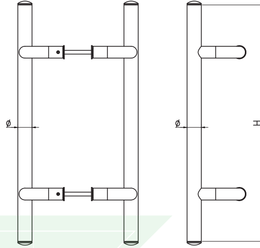
Köşeli "H" kol Curved "H" pull handle
